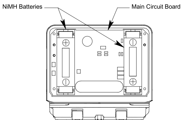
Figure 19 : NiMH Batteries
