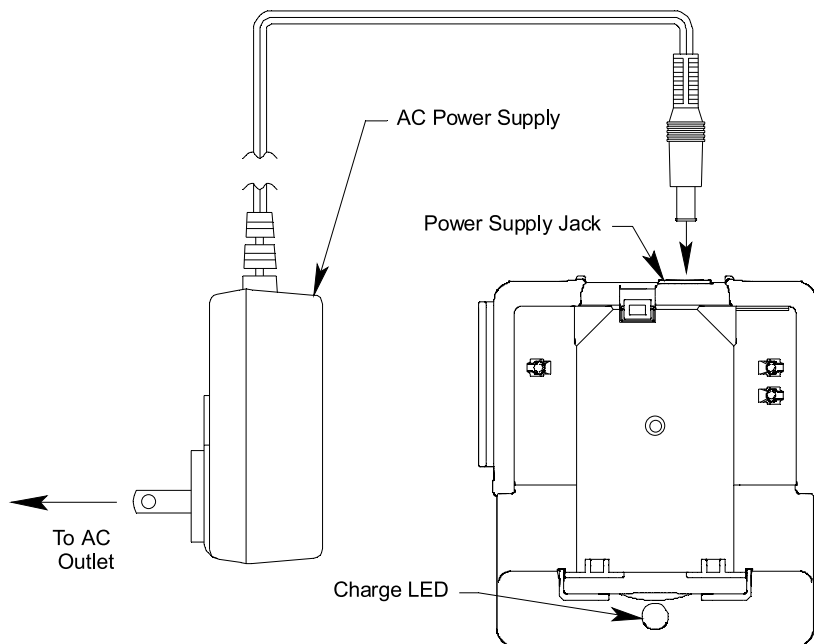
Figure 13 : Calibration Charging Station's AC Adapter
